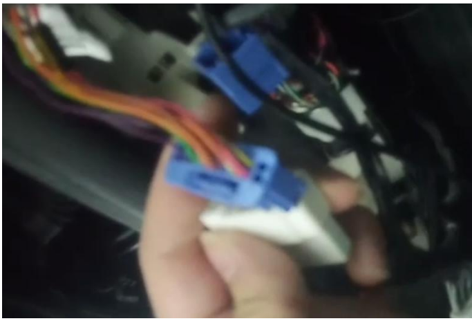
7.主驾 A 柱下方找到蓝色插头拔出转接 Find the blue socket under the A pillar in the driver's cab
