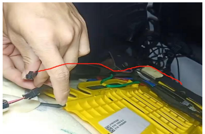
12.插头与安装好后的音响头枕对插，测试完好即可复原 Plug to the installed stereo headrest, recover it after test.
